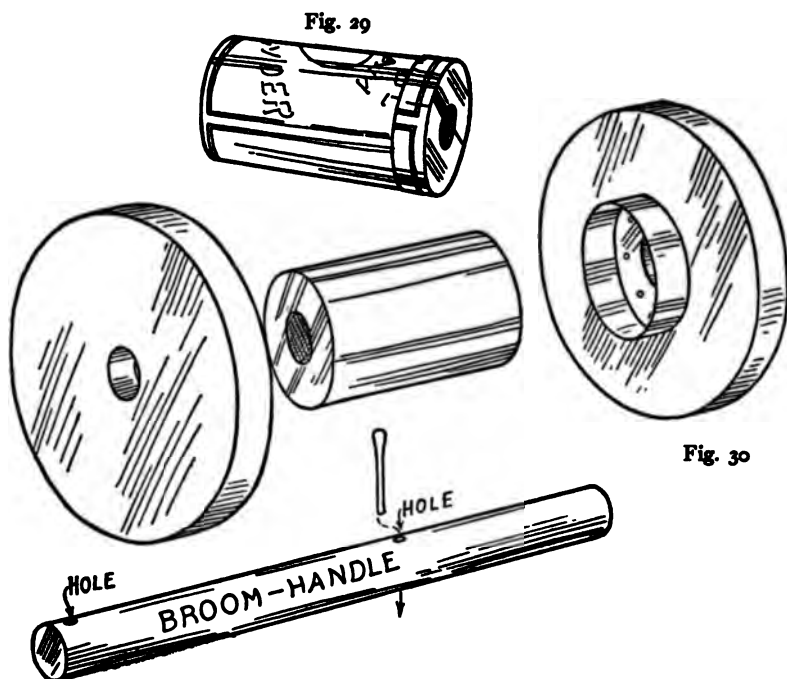
FIGS. 29 and 30. — Details of Hand Kite-Reel.
